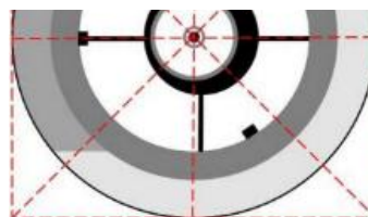
Fast scope (f5 and above ) collimation pattern note the offset
