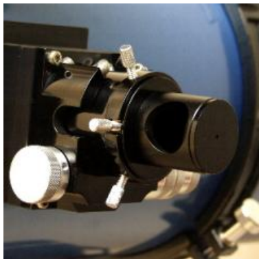
Cheshire collimator in focuser.
